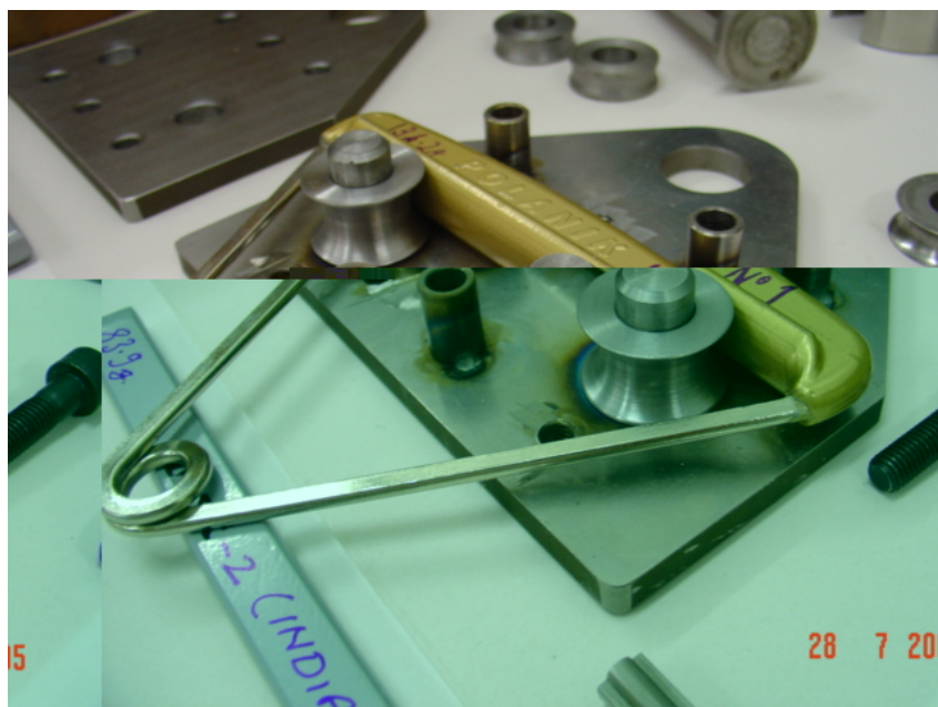
Figure 3. Handle in the Modified Test Fixture (Note the thick ridge along the base of the grip)
